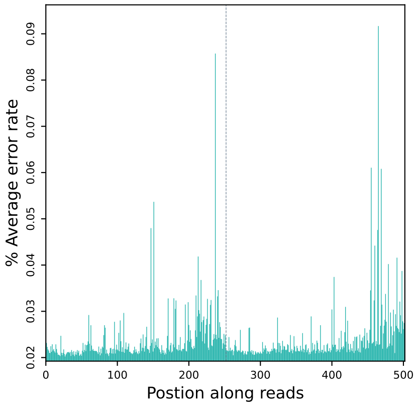
Error rate distribution along reads (R20219)
